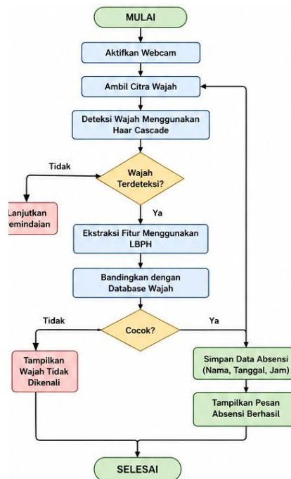
Gambar 1 Flowchart Sistem
