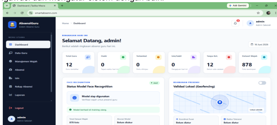
Gambar 4 Dashboard Admin
