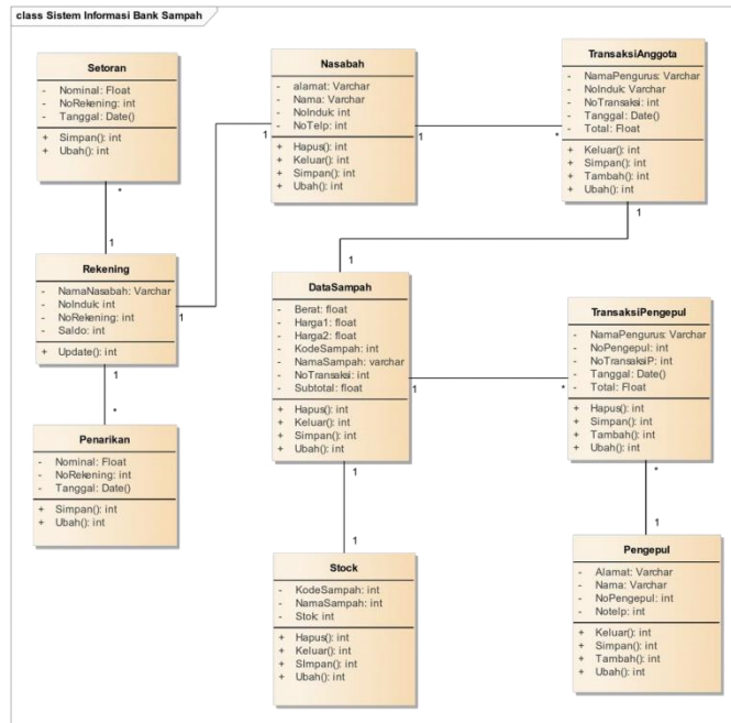
Gbr, 7 Class Diagram SIBAS
