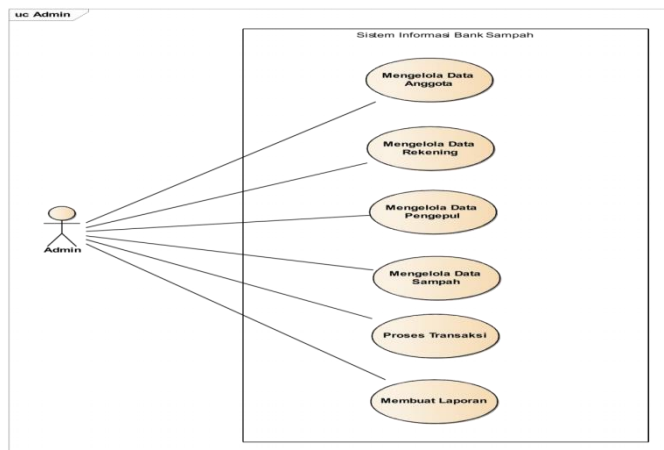
Gbr, 3 Use Case Diagram Admin
