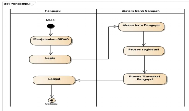
Gbr, 5 Activity Diagram Pengepul
