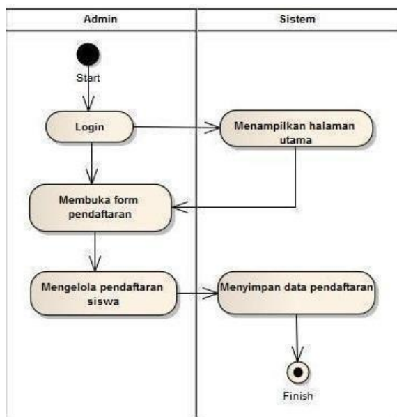
Gambar III. Activity Diagram Halaman Admin
