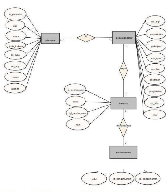
Gambar IV. Entity Relation Diagram
