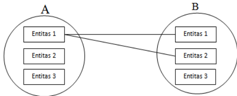
Gambar 2. kardinalitas One-to-Many
