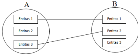
Gambar 1. kardinalitas One-to-One
