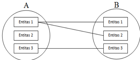
Gambar 3. kardinalitas Many-to-Many
