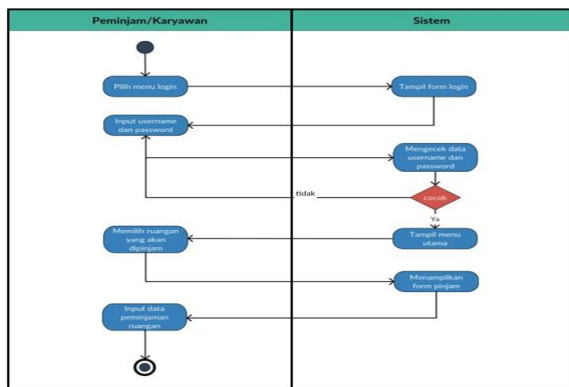
Gambar 2 Activity Diagram peminjaman ruang meeting
