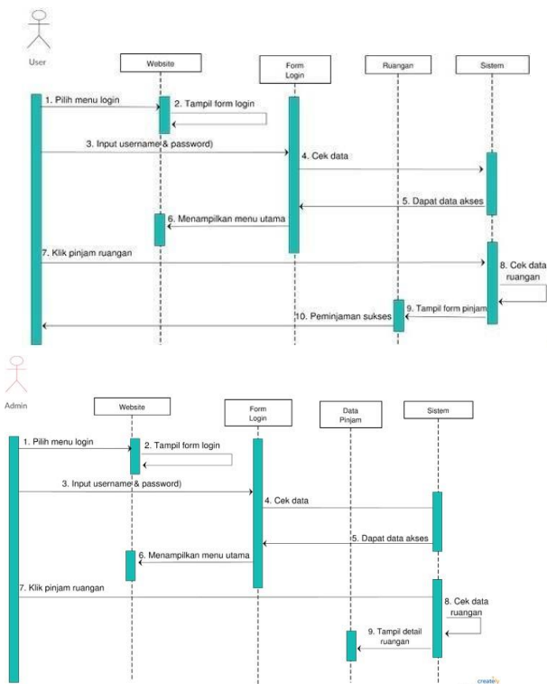
Gambar 3 Sequence Diagram User
