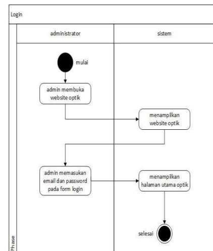
Gambar 5. Diagram activity login
