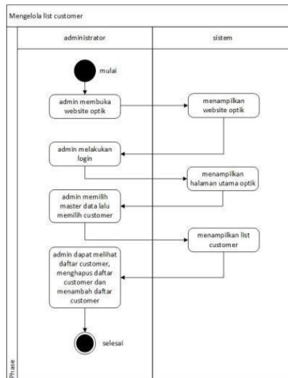
Gambar 6. Diagram activity list customer
