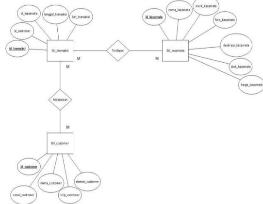
Gambar 19. Entity Relationship Diagram
