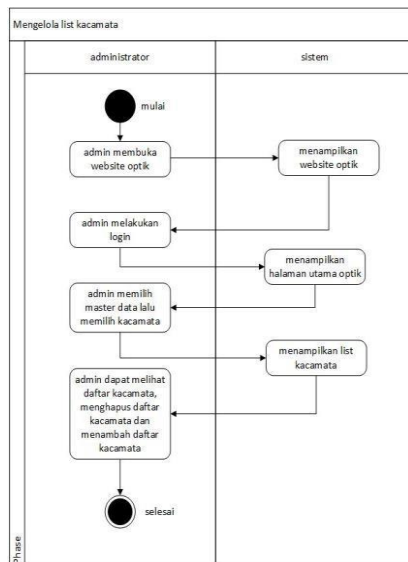
Gambar 7. Diagram activity listacamata
