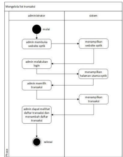
Gambar 9. Diagram activity list transaksi
