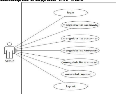
Gambar 3. Use Case Diagram Sistem
