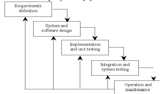
Gambar 1. Waterfall Model
