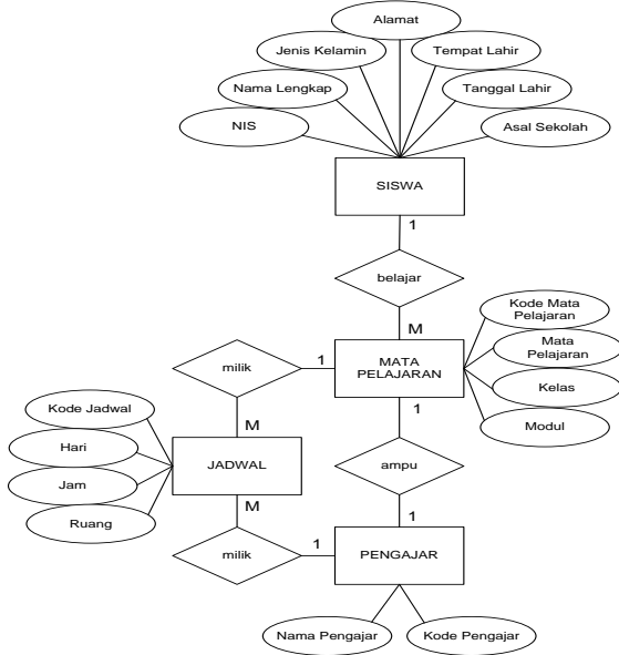
Gambar 6. Database Bimbel
