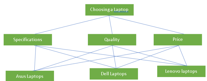
Fig.2 Hierarchical Structure
