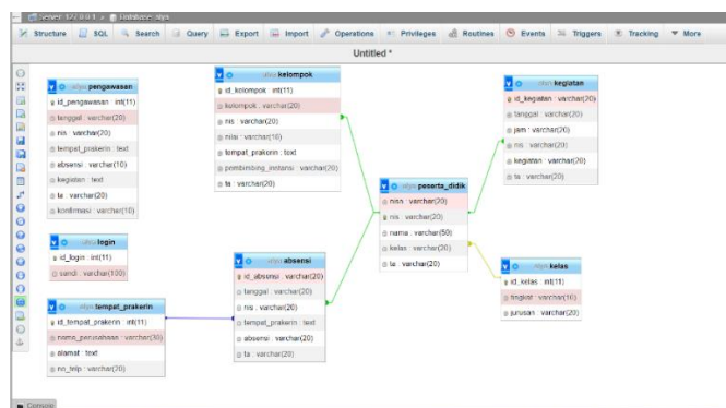
Figure 5. Entity Diagram Relationship
