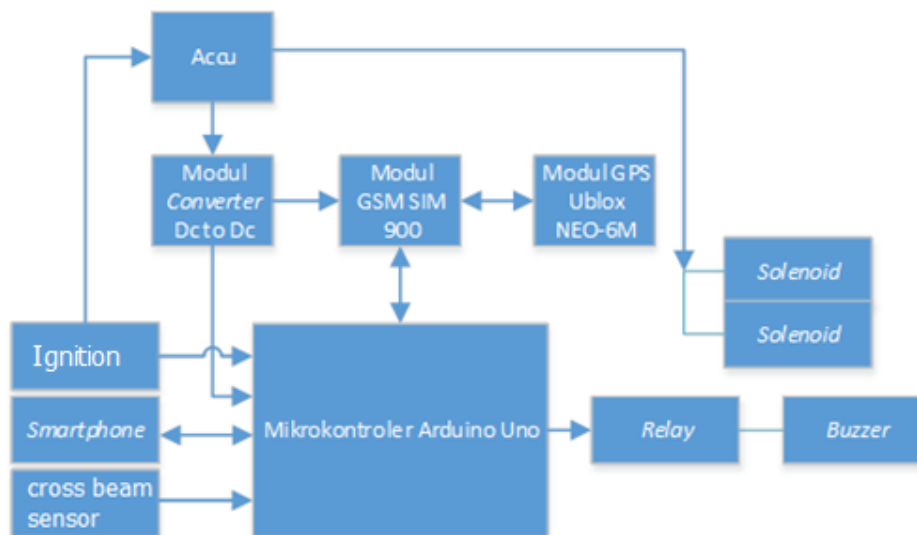
Figure 1 System Design Block Diagram
