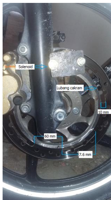
Figure 13 Results of Front Disc Design
