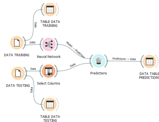
Fig 2. System Design Process in Data Mining
