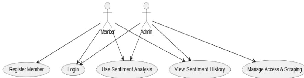
Figure 2. Use Case Diagram
