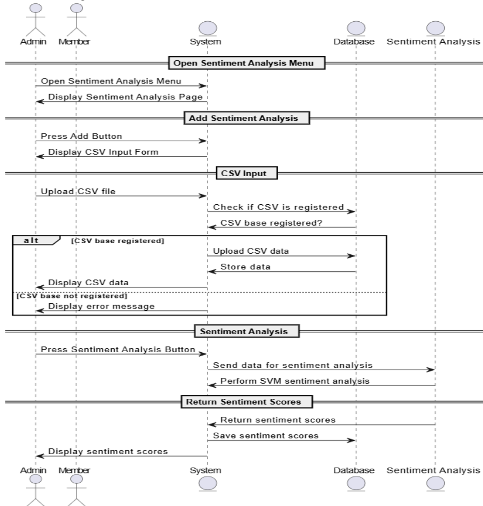
Figure 6. Sentiment Analysis Activity Diagram
