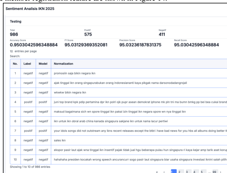
Figure 14. Sentiment Analysis Testing Results
