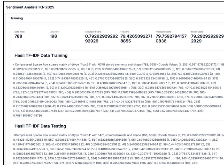
Figure 13. Sentiment Analysis Training Results
