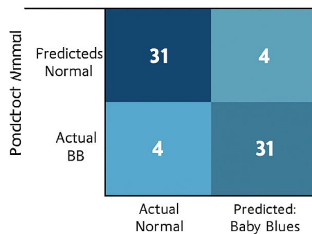
Figure 2. Confusion Matrix (K=5)
